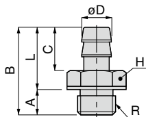
Metric thread
